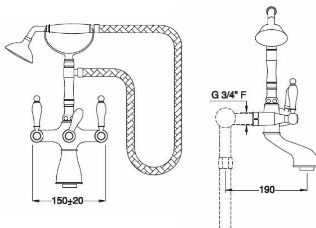
DISEGNO TECNICO/TECHNICAL DRAWING/DESSIN TECHNIQUE
