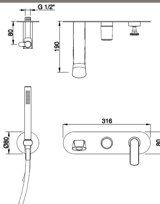
DISEGNO TECNICO/TECHNICAL DRAWING/DESSIN TECHNIQUE
